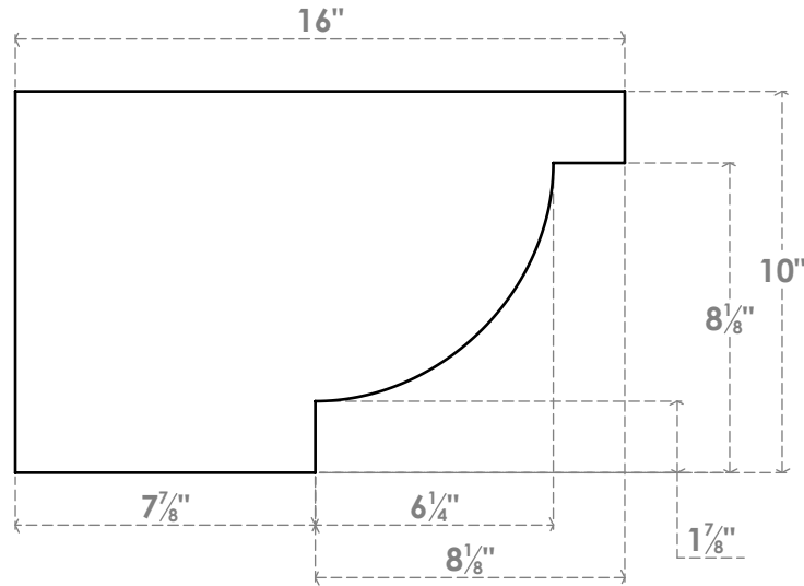
SIDE PROFILE
